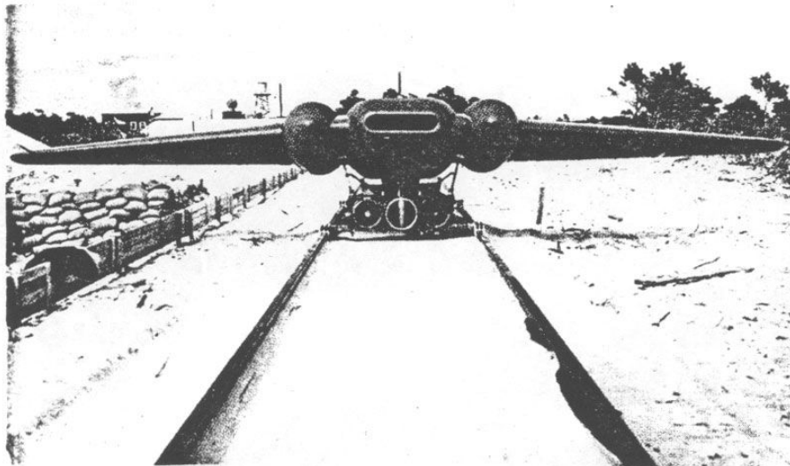
A JB-1 sits on one of the 1,000+ Northrop designed launchers on a 50 foot track at Eglin AFB, Florida. The central intake housed two small jet engines with separate exhausts on either side of the vertical fin. Pods on each wing housed 1,000 lb bombs. The JB-1 vehicle first flew as a manned powerless glider. The JB-1 program was terminated because of problems of engine-aircraft compatibility. The outer wing sections were then used with the new ramjet powered center section to create the JB-10. (Ref.2)
